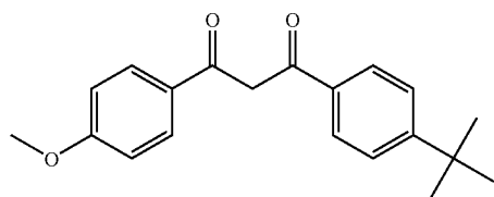
4-(1,1-dimethylethyl)-4'-methoxydibenzoylmethane PARSOL 1789
