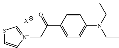
3-[2-(4-diethylaminophenyl)-2-oxoethyl]thiazolium salt
